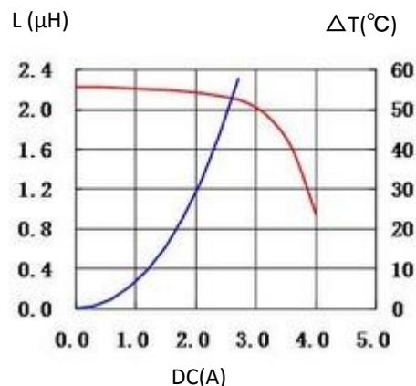
3. CD4018MBDS-2R2MC
