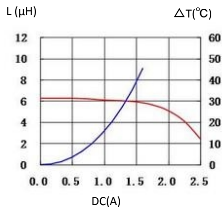
6. CD4018MBDS-6R8MC
