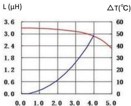
2. CD5040MBDS-3R3NC
