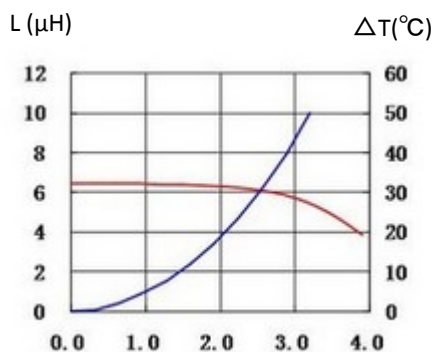
4. CD5040MBDS-6R8NC
