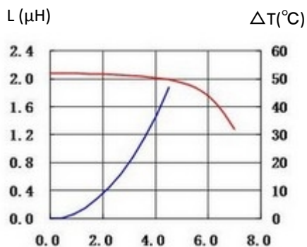
1. CD5040MBDS-2R2NC
