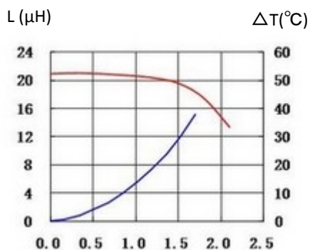
7. CD5040MBDS-220MC
