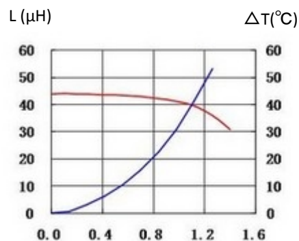
9. CD5040MBDS-470MC
